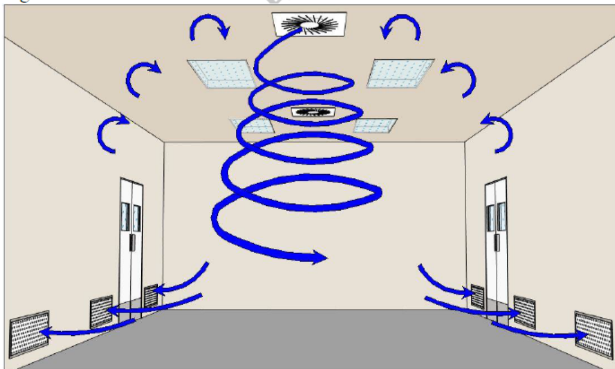
Figure 20. Swirl diffuser
